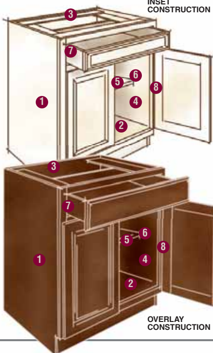
INSET CONSTRUCTION
